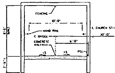
TYPICAL SECTION NO SCALE
