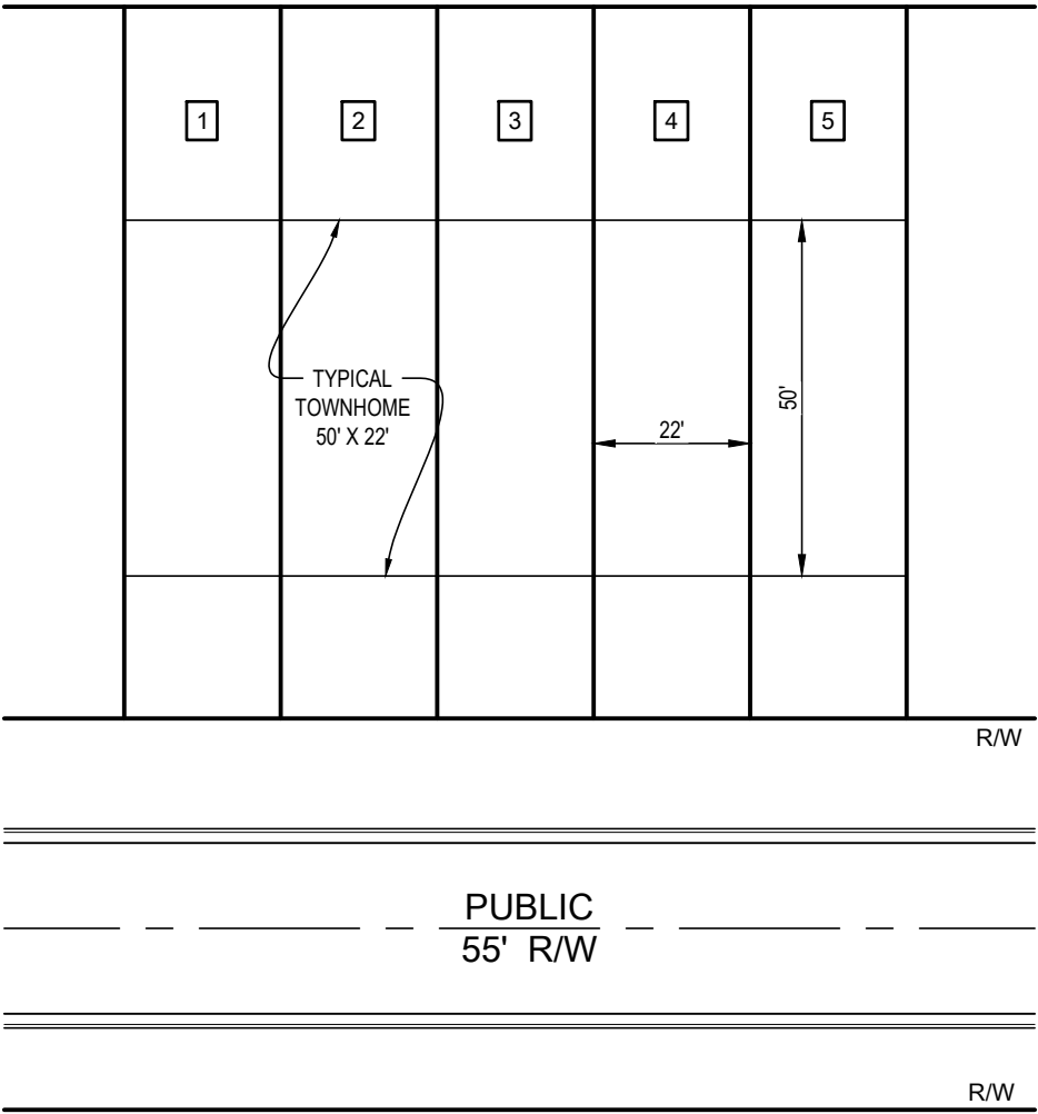
TYPICAL LOT LAYOUT
