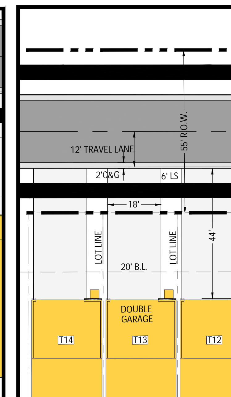
TYPICAL TOWNHOME LAYOUT N.T.S.
