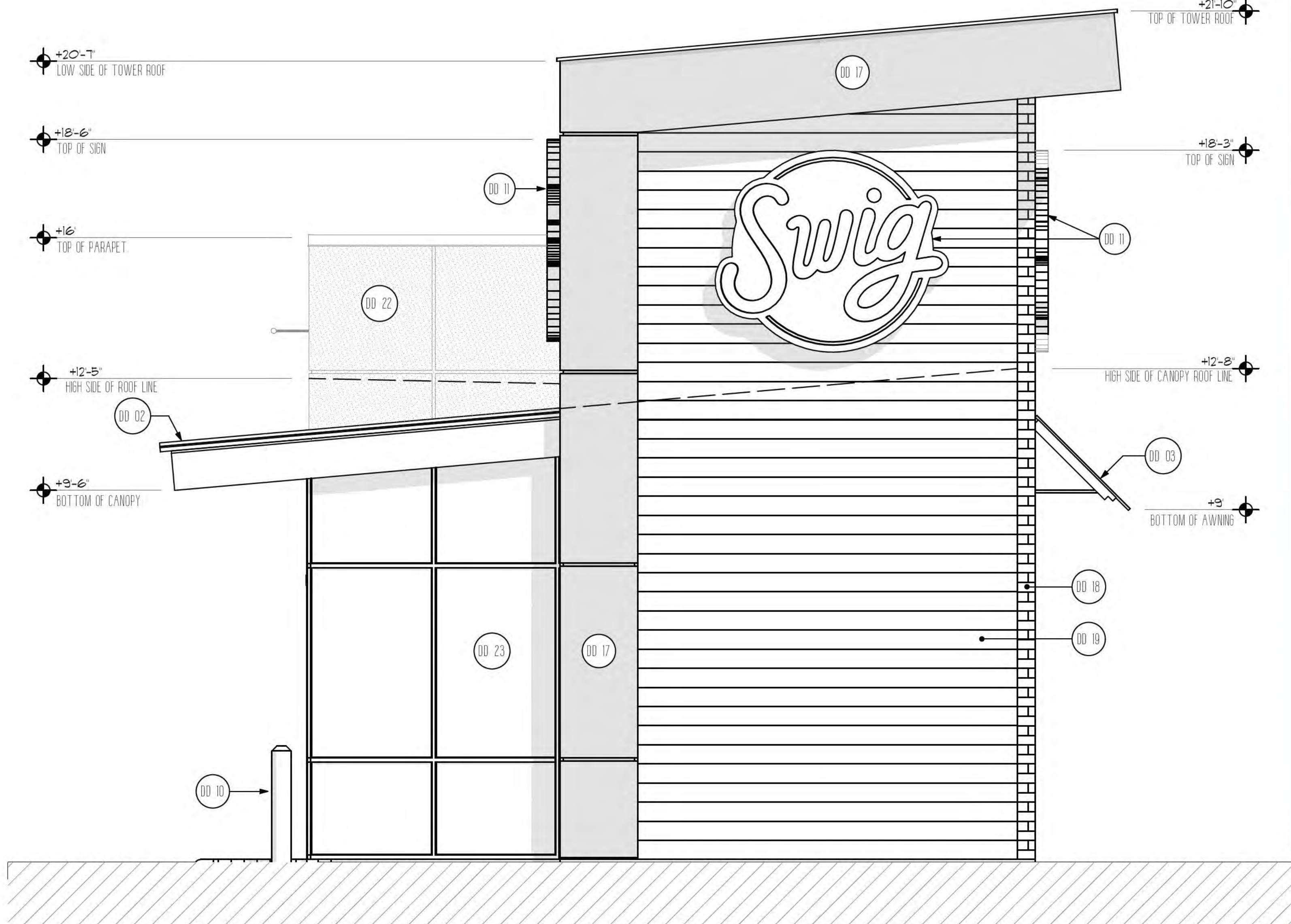
1 SIDE ELEVATION
