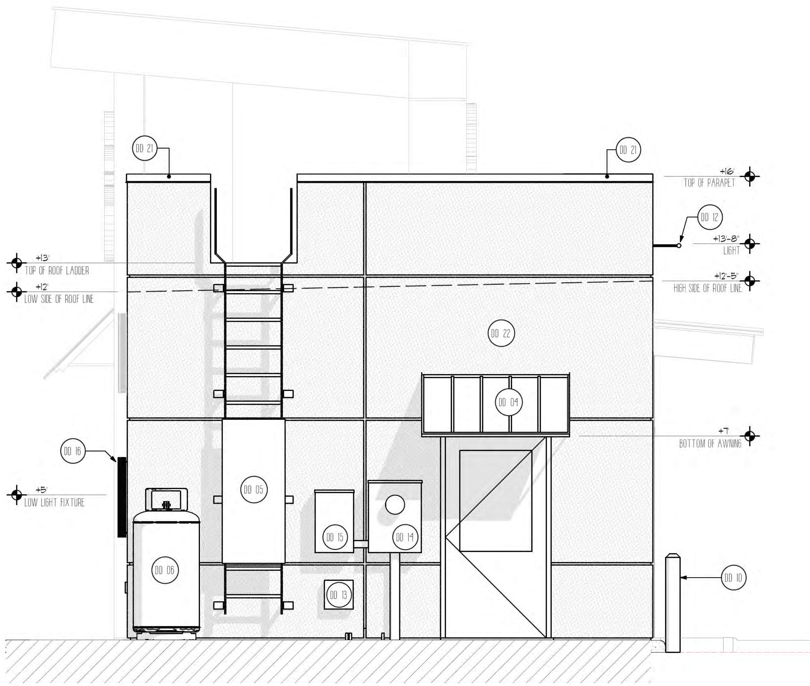
2 BACK ELEVATION
