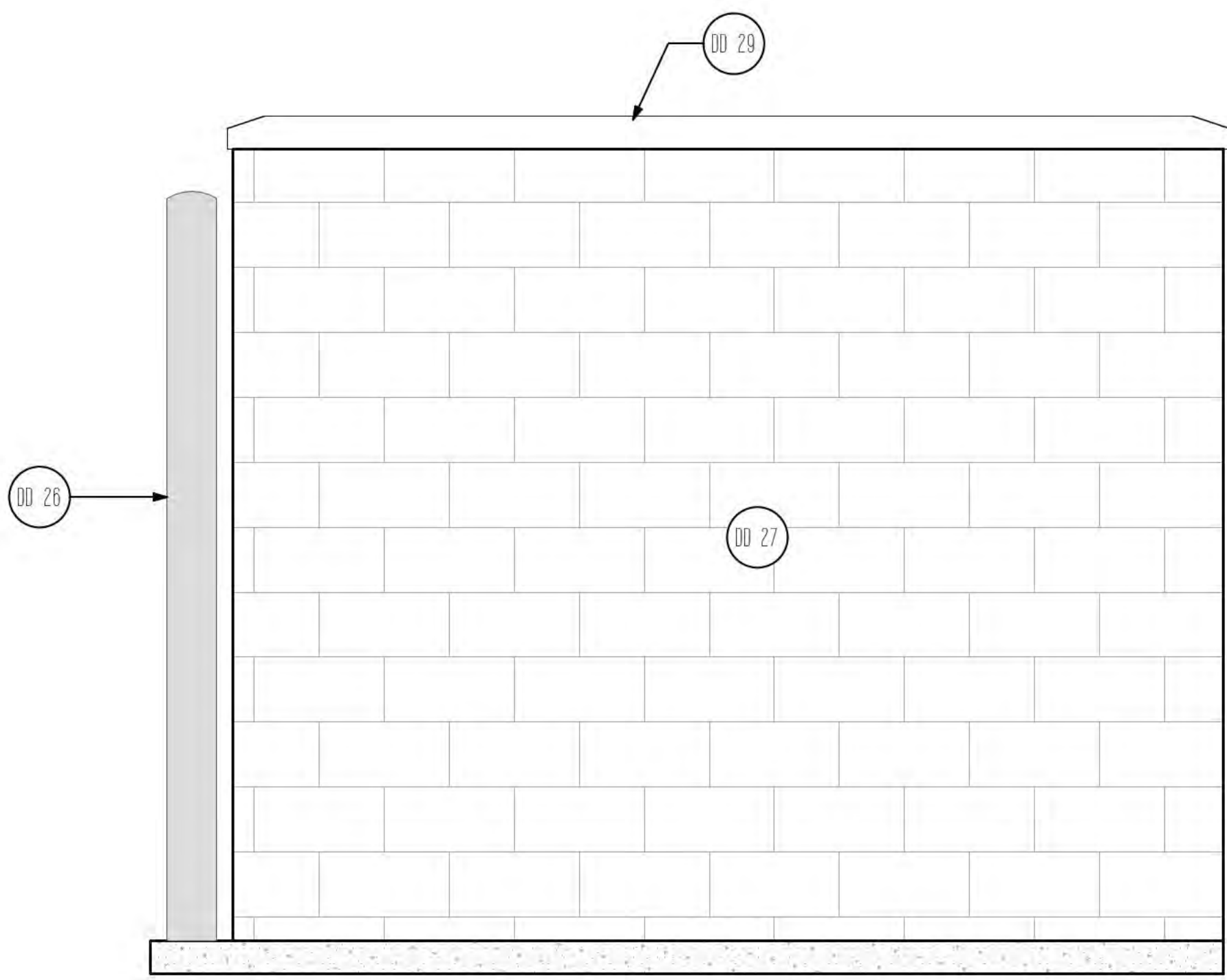
SIDE ELEVATION
