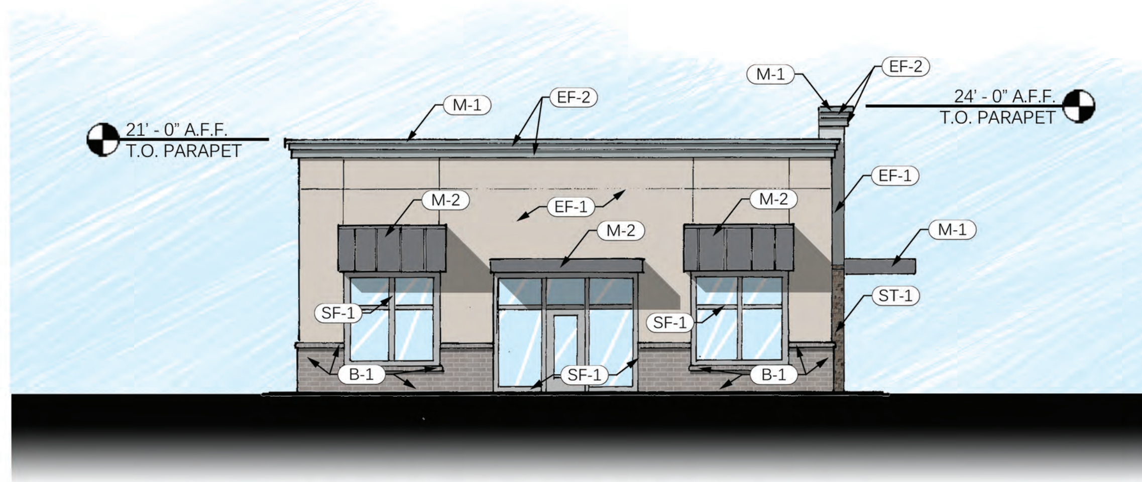
PATIO ELEVATION
